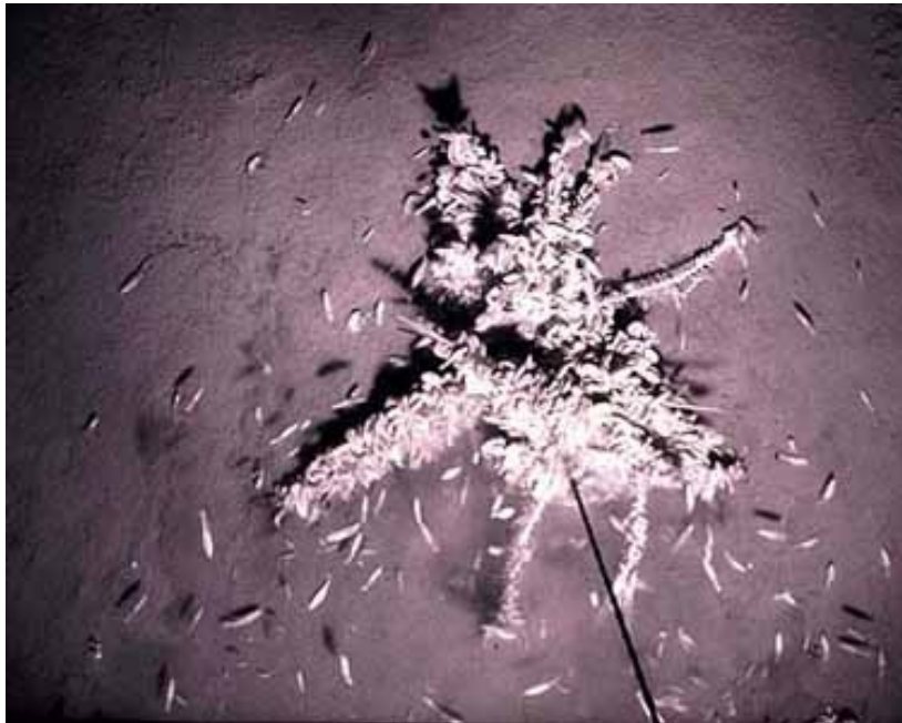
The lysianassoid Hirondellea gigas swarming bait at 9605m in the Philippine Trench (Photo R. R. Hessler, SIO)
